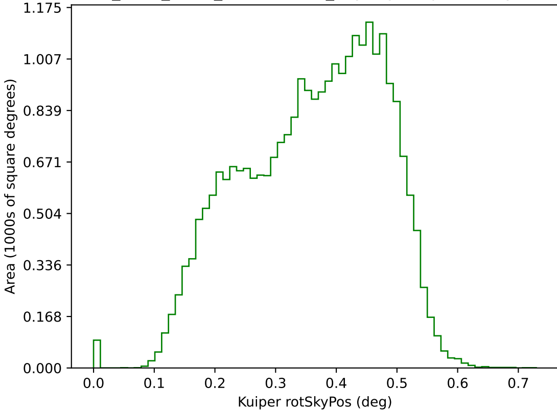
roll_mid1_const_season2v3.3_10yrs g: Kuiper rotSkyPos
