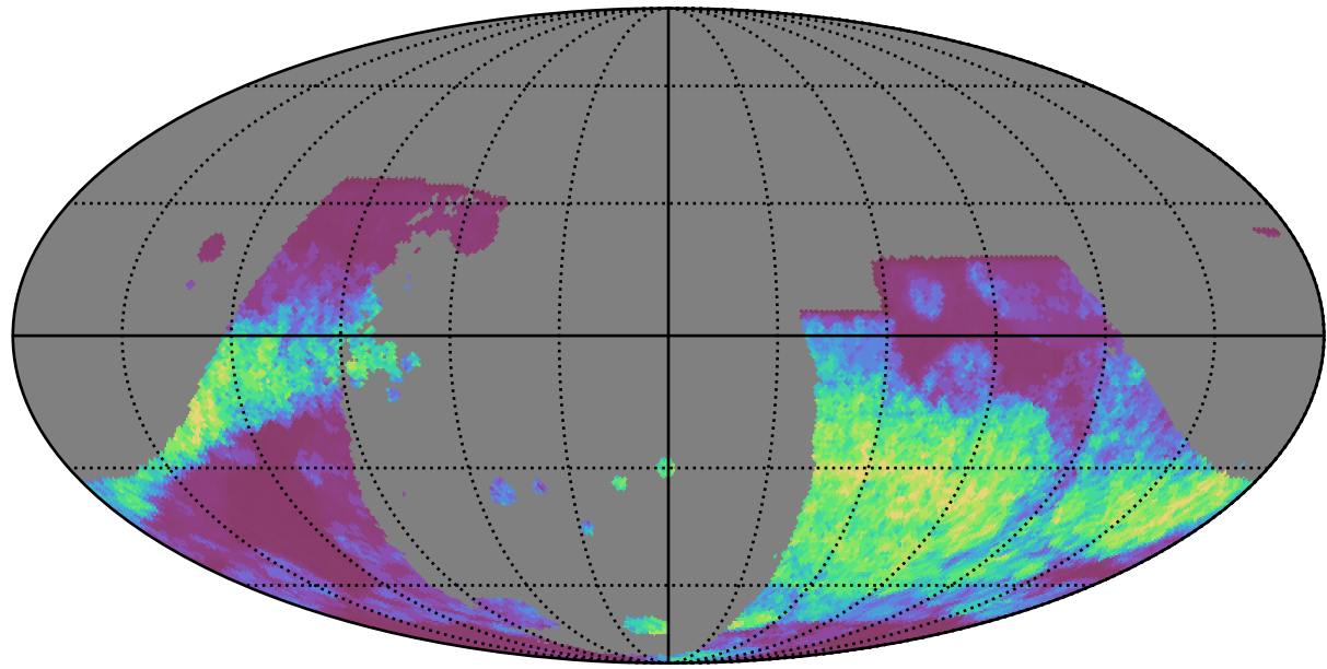
0.0 0.1 0.2 0.3 0.4 0.5 0.6 0.7 0.8 0.9 1.0 GalPlaneSeasonGapsTimescales_combined_map_Tau_55_0 (MJD mag)
