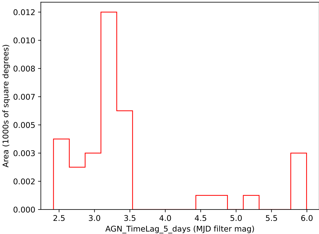
roll_mid1_const_season2v3.3_10yrs i band: AGN_TimeLag_5_days
