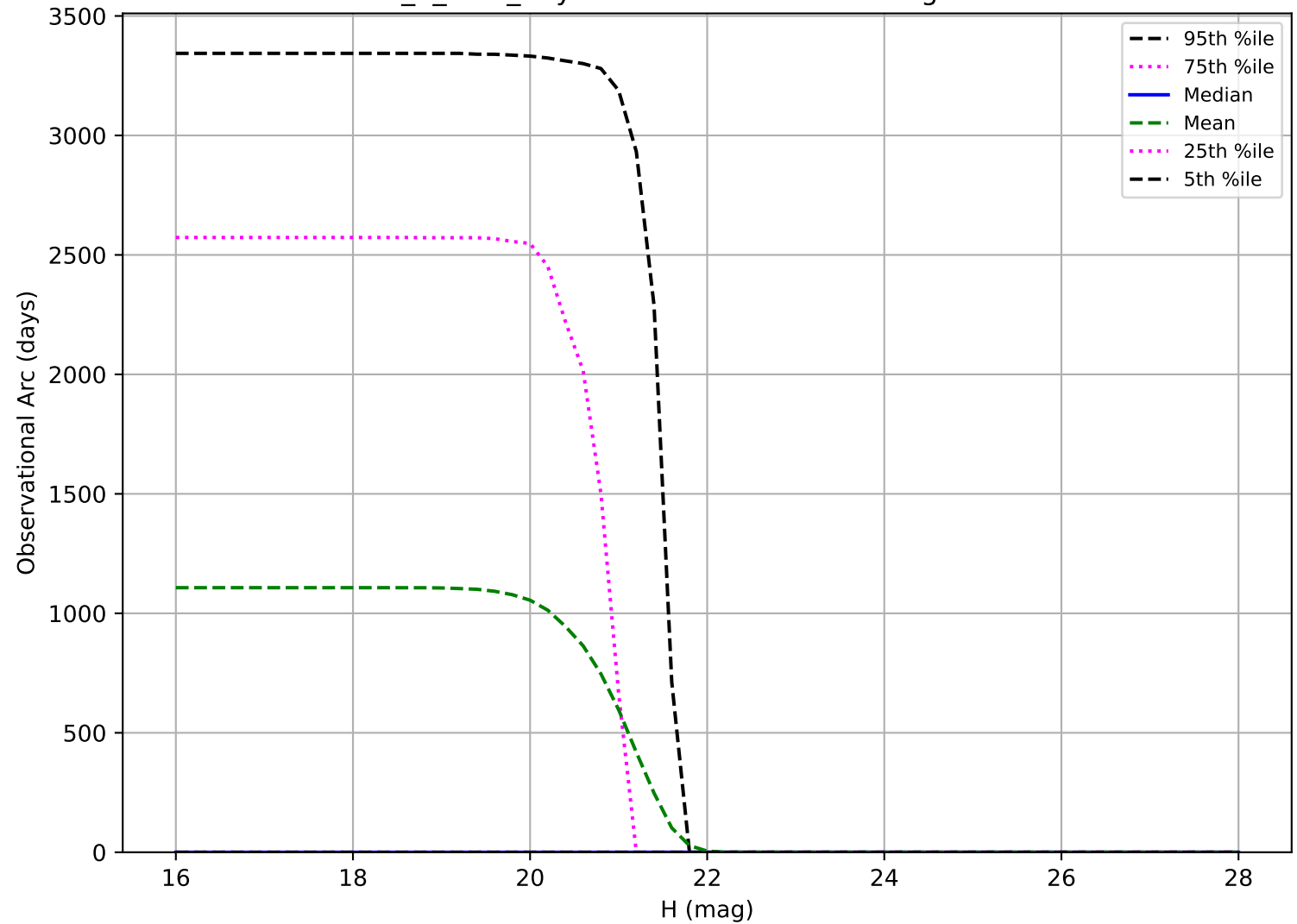
roll_3_v3.4_10yrs: Observational Arc Length Vatra
