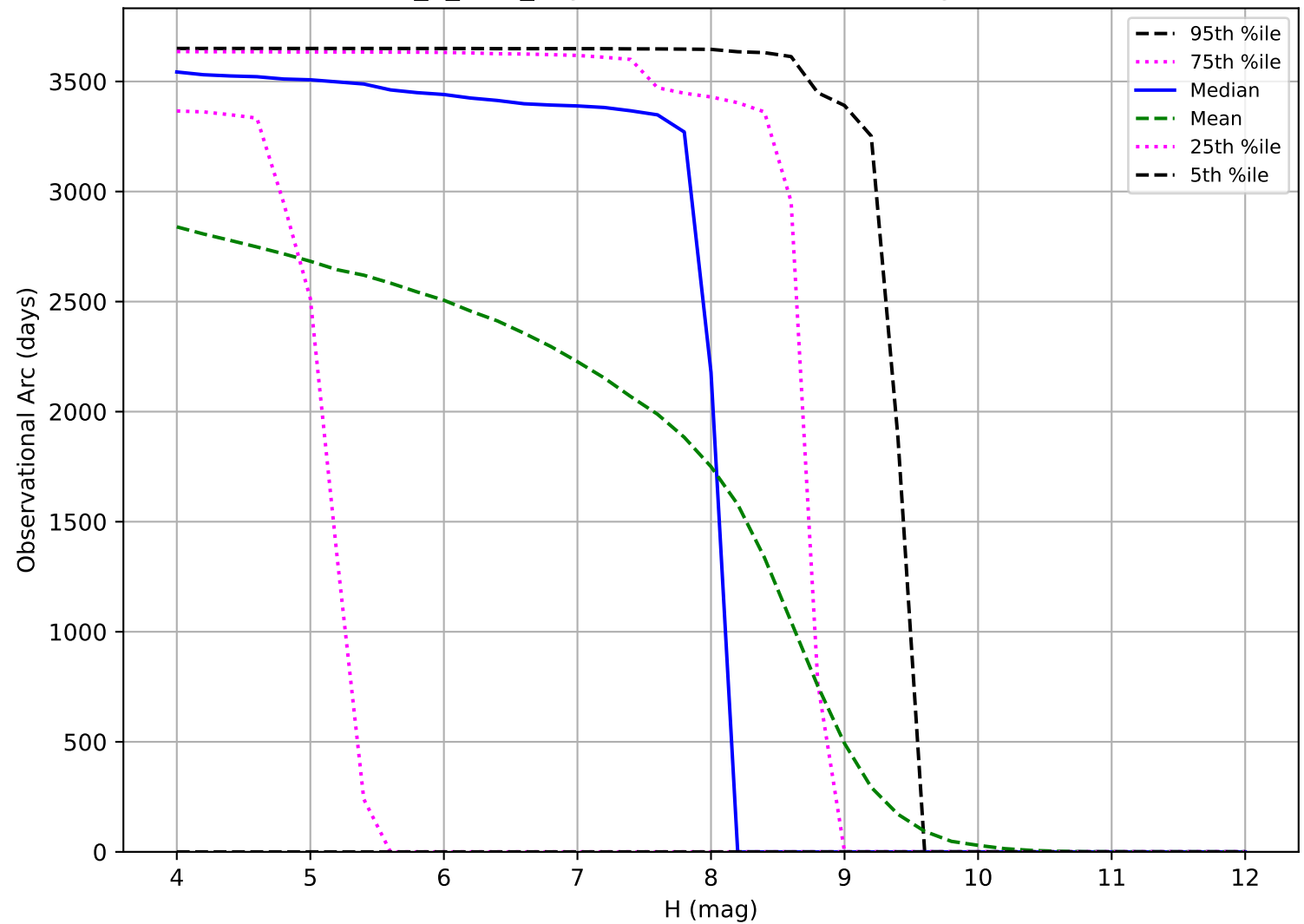
roll_3_v3.4_10yrs: Observational Arc Length TNO
