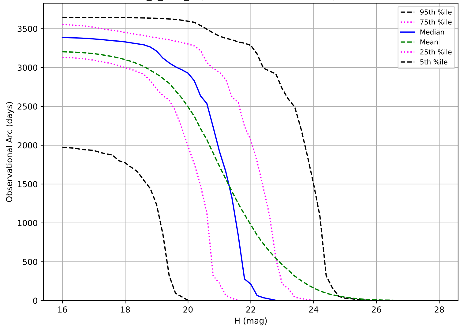
roll_3_v3.4_10yrs: Observational Arc Length PHA
