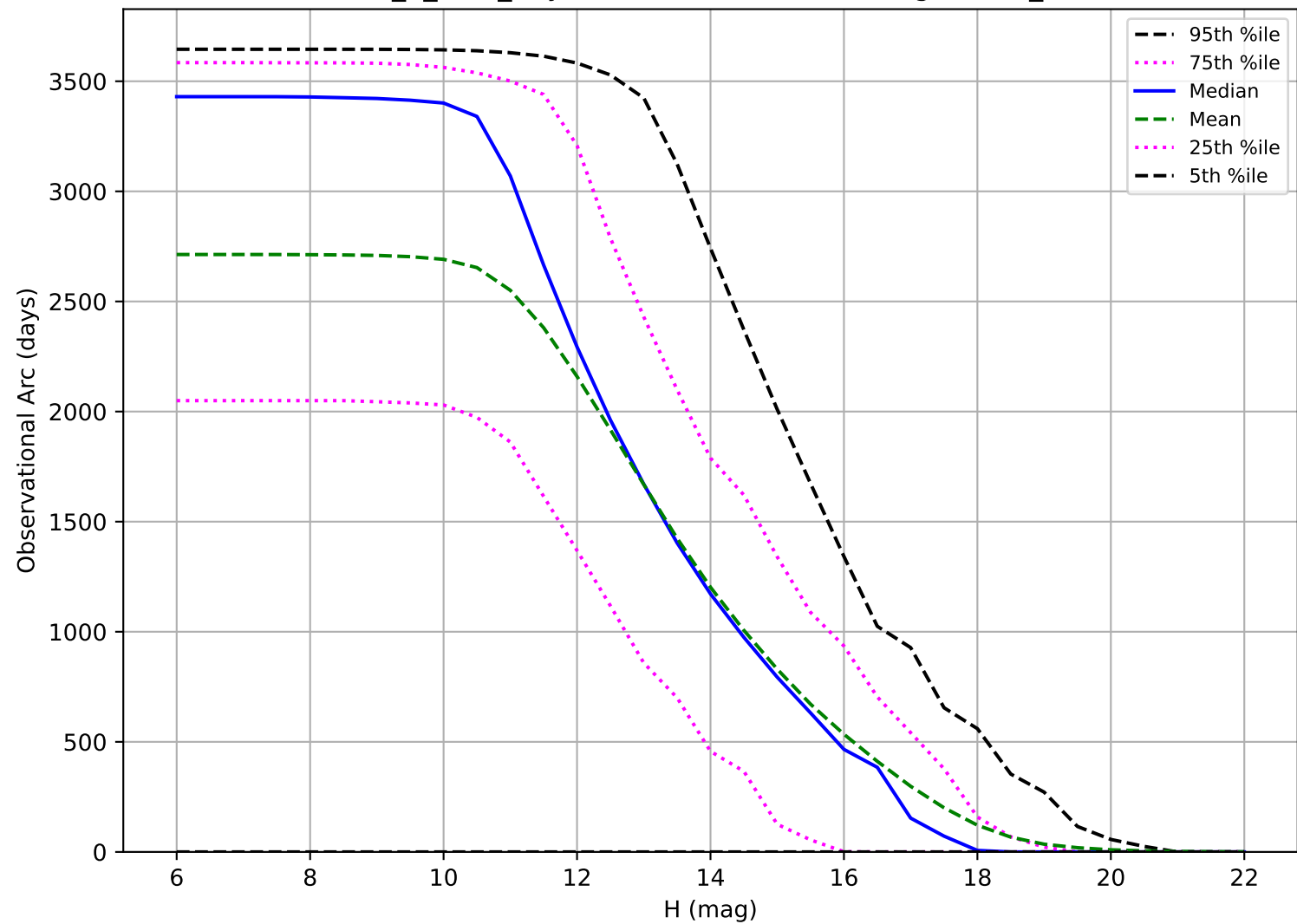
roll_3_v3.4_10yrs: Observational Arc Length OCC_r5
