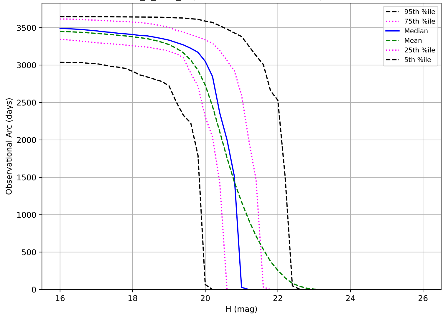
roll_3_v3.4_10yrs: Observational Arc Length MBA
