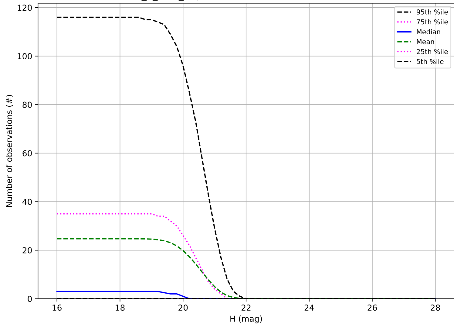
roll_3_v3.4_10yrs: Number of observations Vatira
