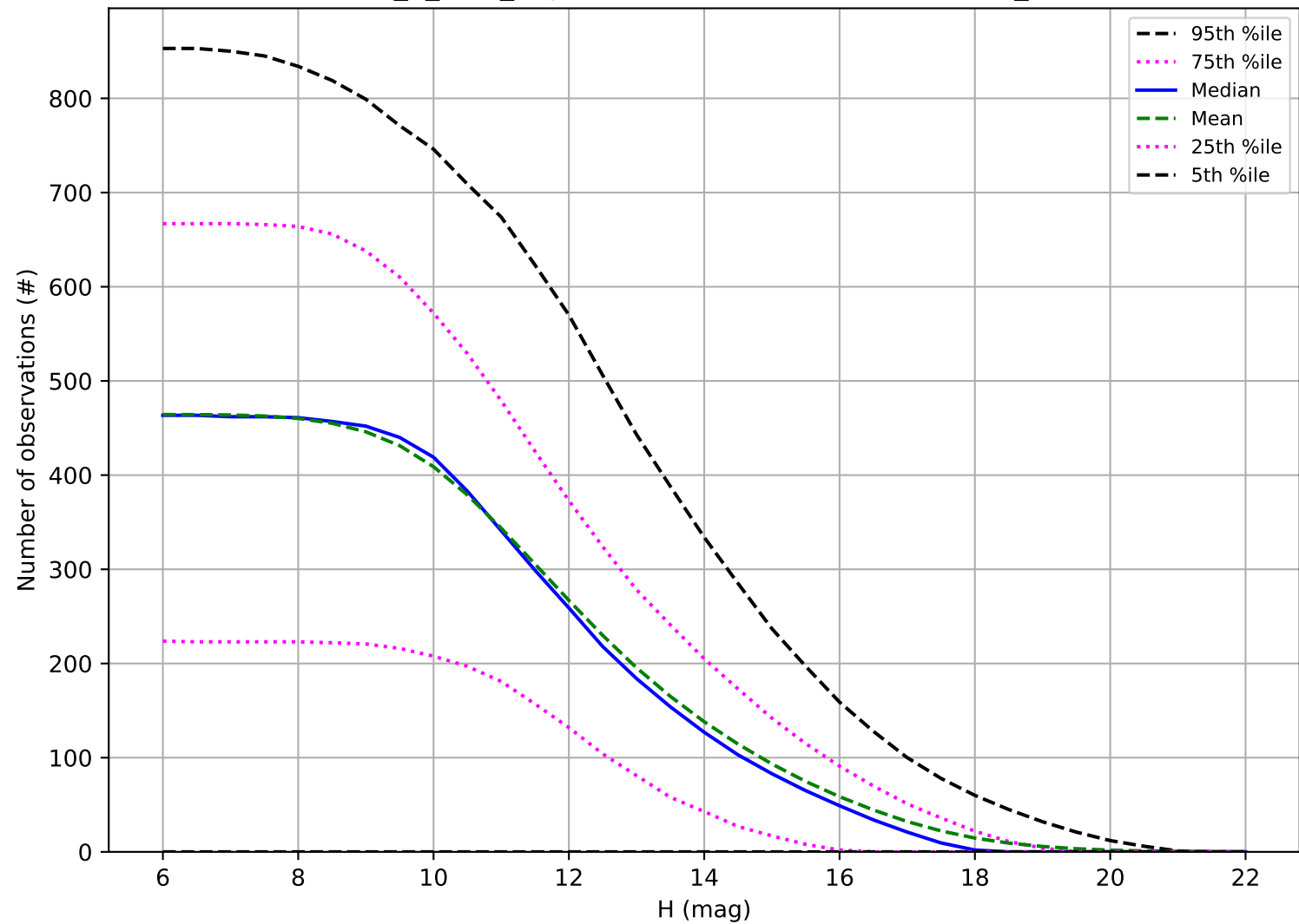
roll_3_v3.4_10yrs: Number of observations OCC_r5
