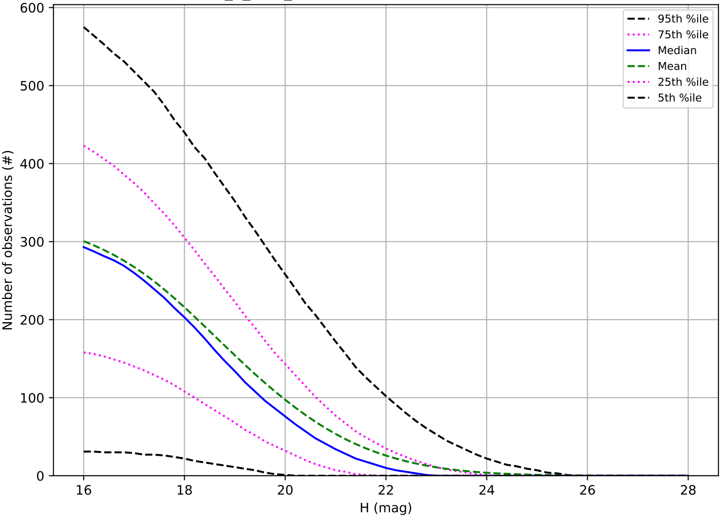
roll_3_v3.4_10yrs: Number of observations NEO
