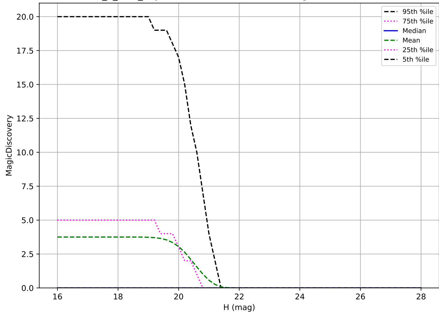
roll_3_v3.4_10yrs: Vatira 6 detections in 60 nights detection loss
