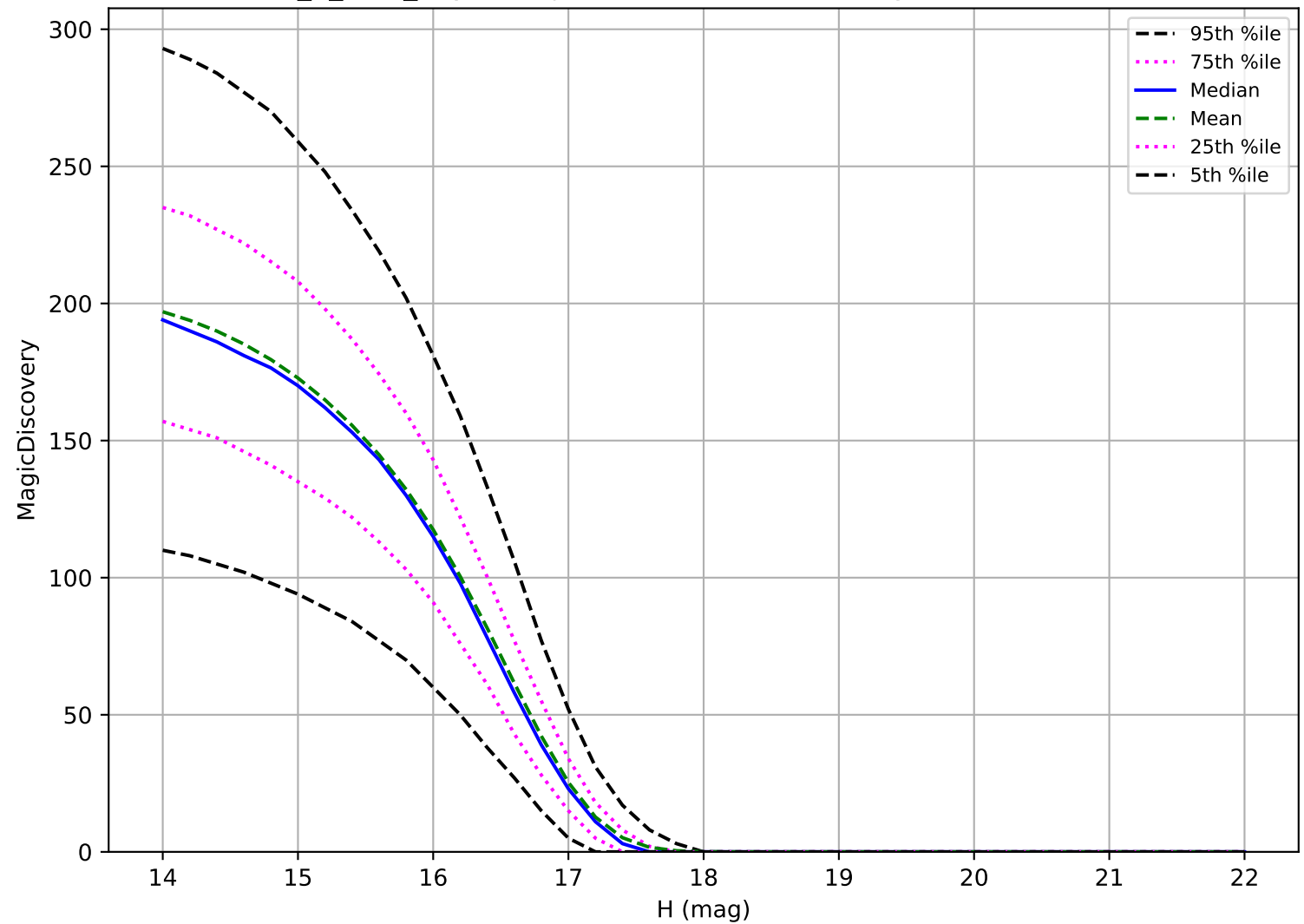
roll_3_v3.4_10yrs: Trojan 6 detections in 60 nights detection loss
