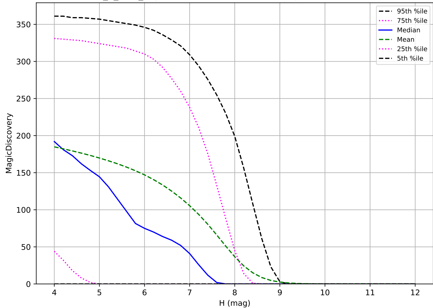
roll_3_v3.4_10yrs: TNO 6 detections in 60 nights detection loss
