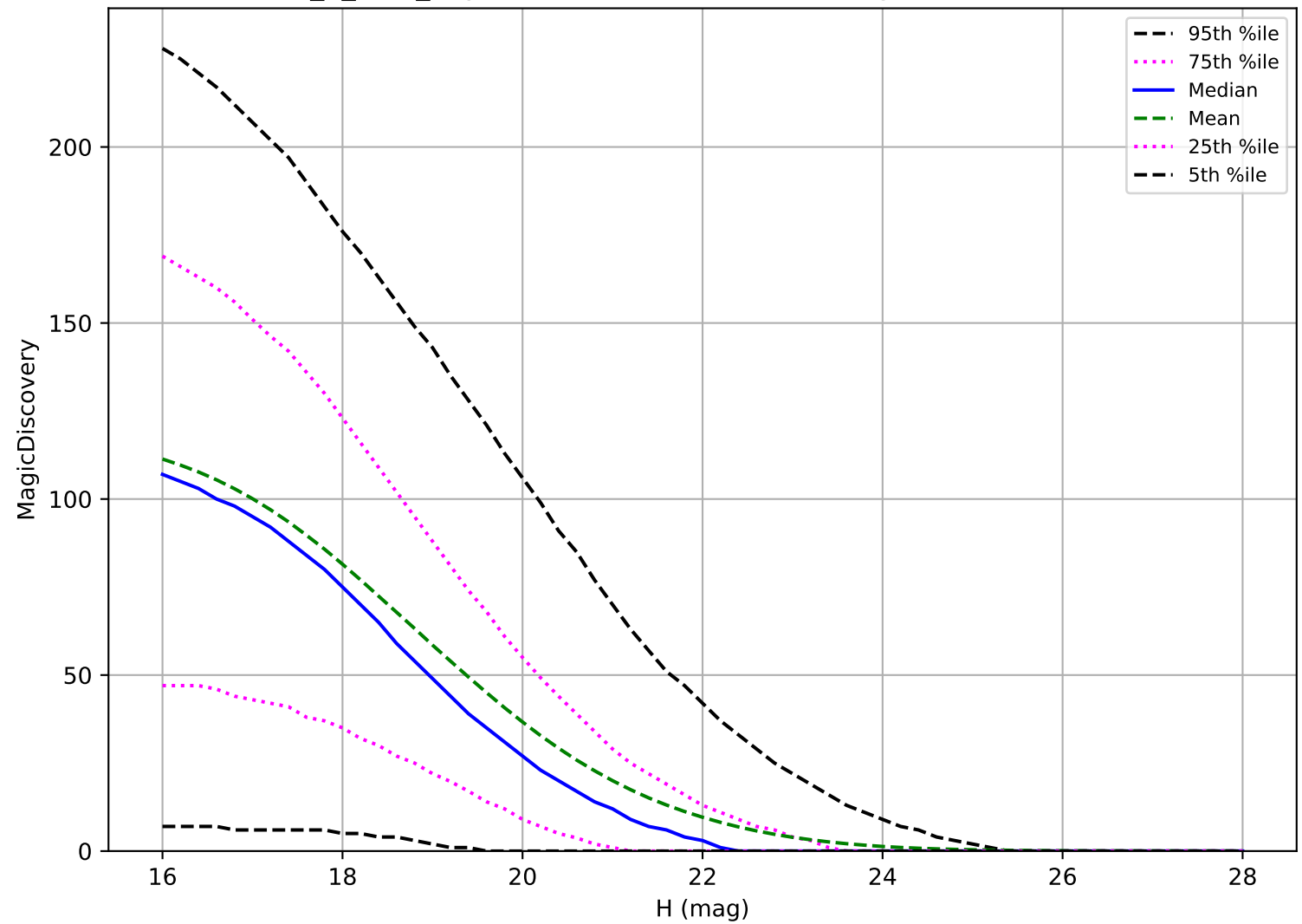
roll_3_v3.4_10yrs: PHA 6 detections in 60 nights detection loss
