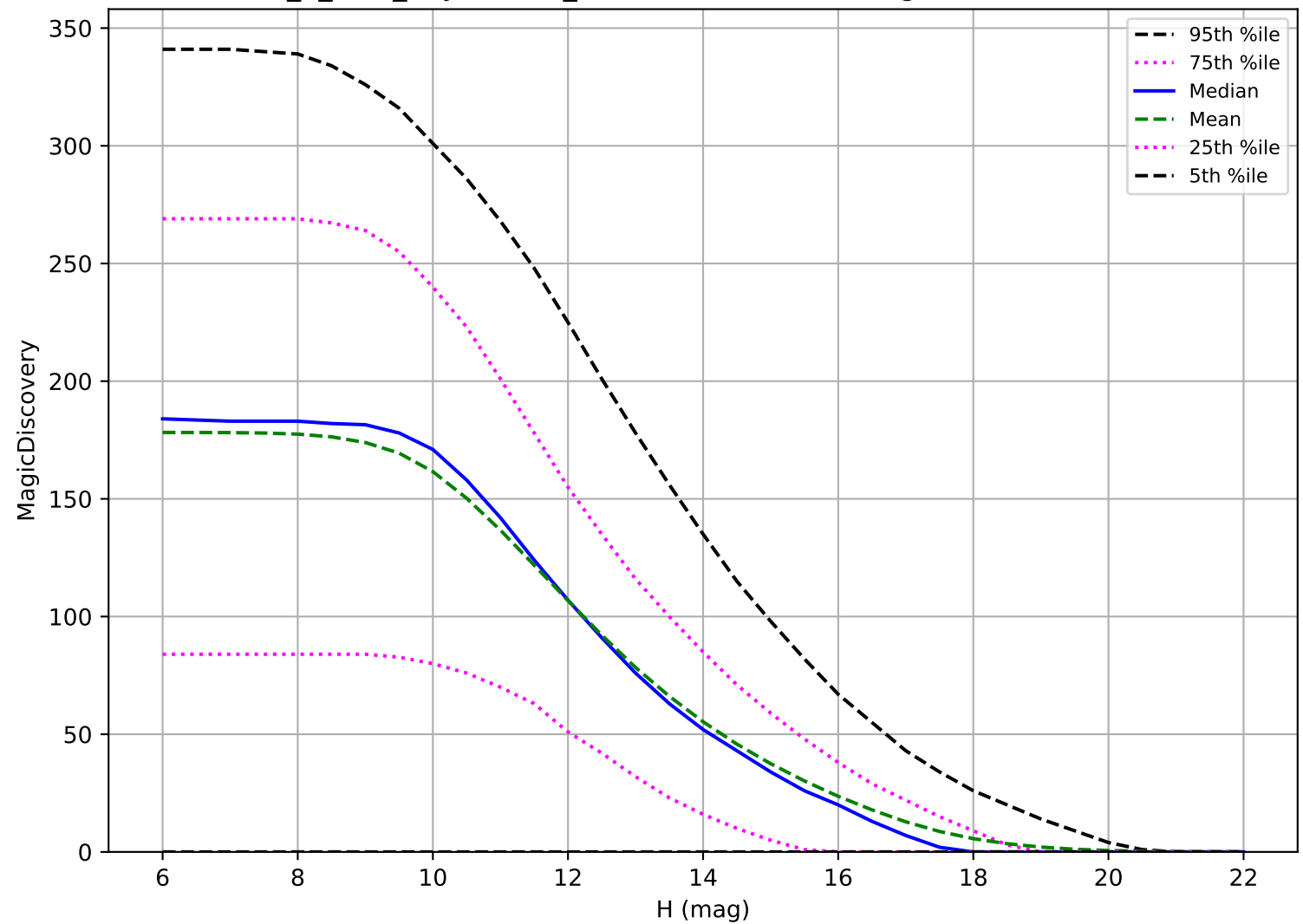
roll_3_v3.4_10yrs: OCC_r5 6 detections in 60 nights detection loss
