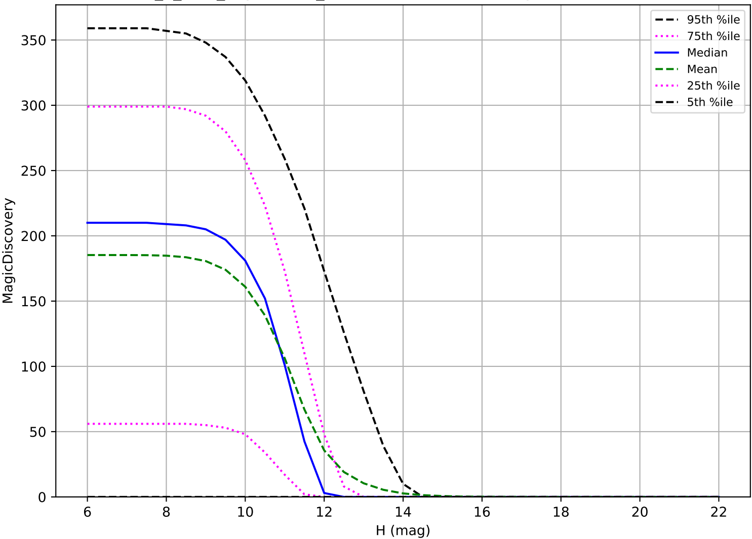
roll_3_v3.4_10yrs: OCC_r20 6 detections in 60 nights detection loss
