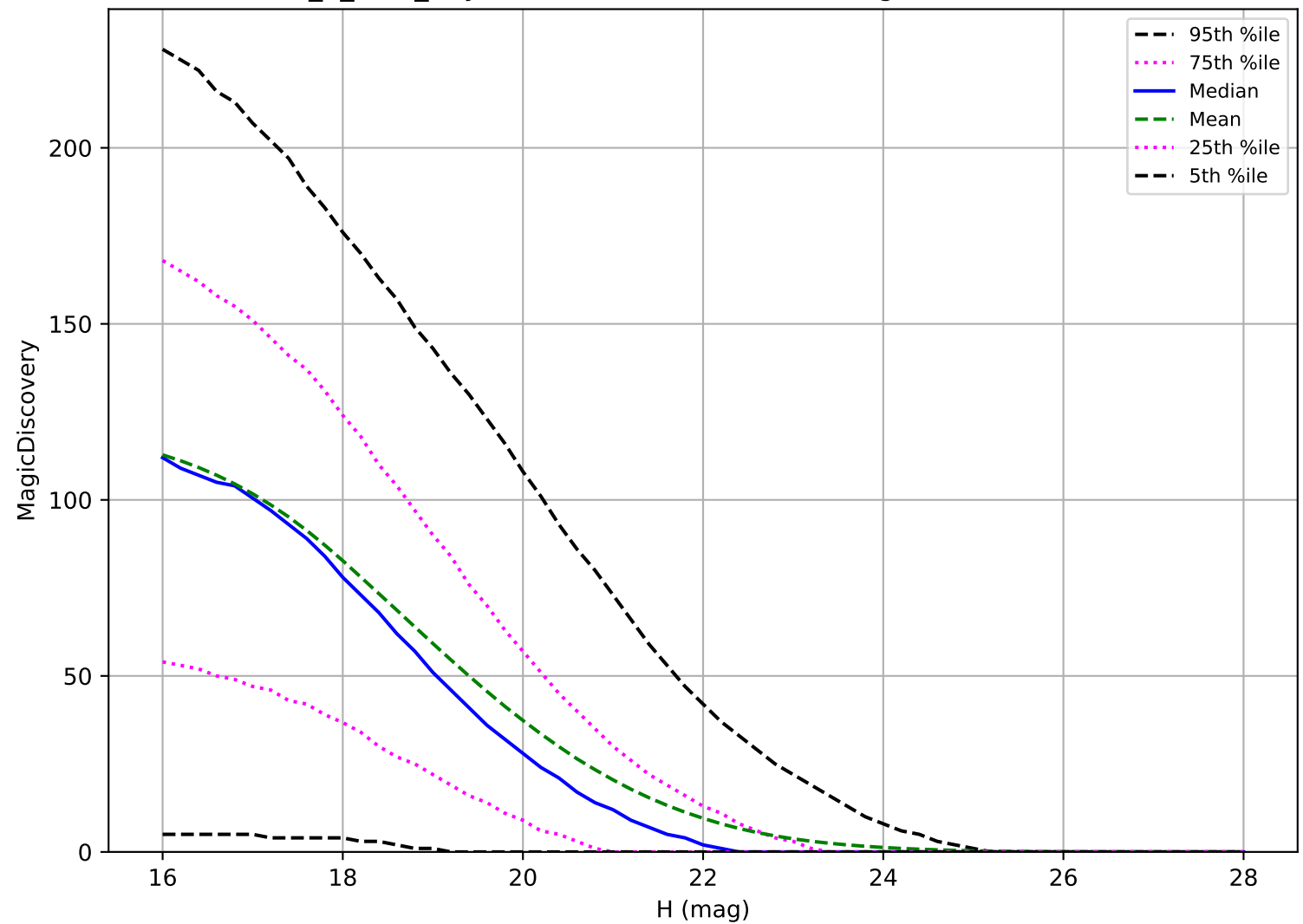
roll_3_v3.4_10yrs: NEO 6 detections in 60 nights detection loss
