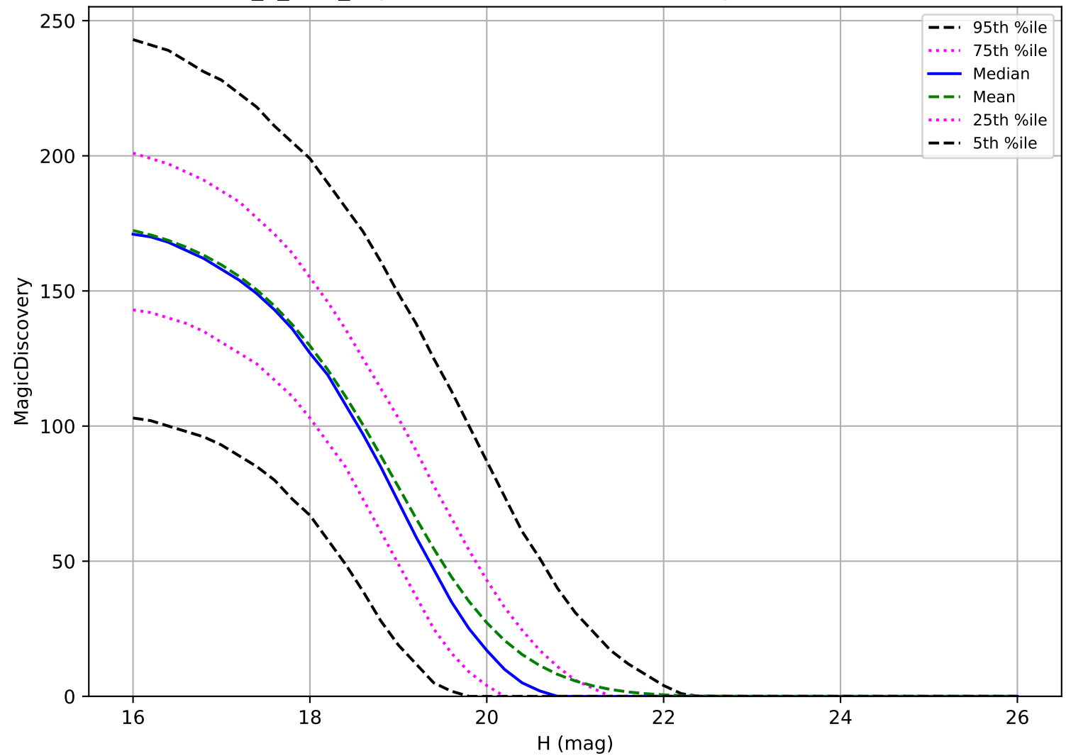
roll_3_v3.4_10yrs: MBA 6 detections in 60 nights detection loss
