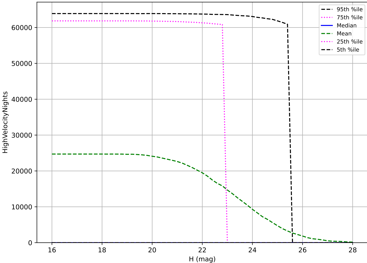
roll_3_v3.4_10yrs: PHA High velocity pair detection loss
