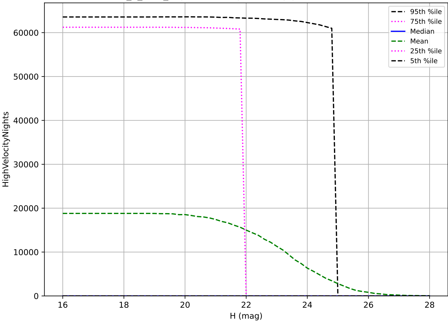
roll_3_v3.4_10yrs: NEO High velocity pair detection loss
