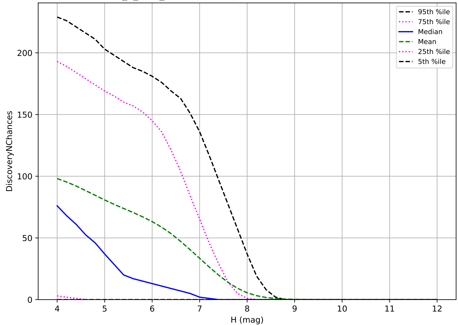
roll_3_v3.4_10yrs: TNO 3 pairs in 15 nights detection loss
