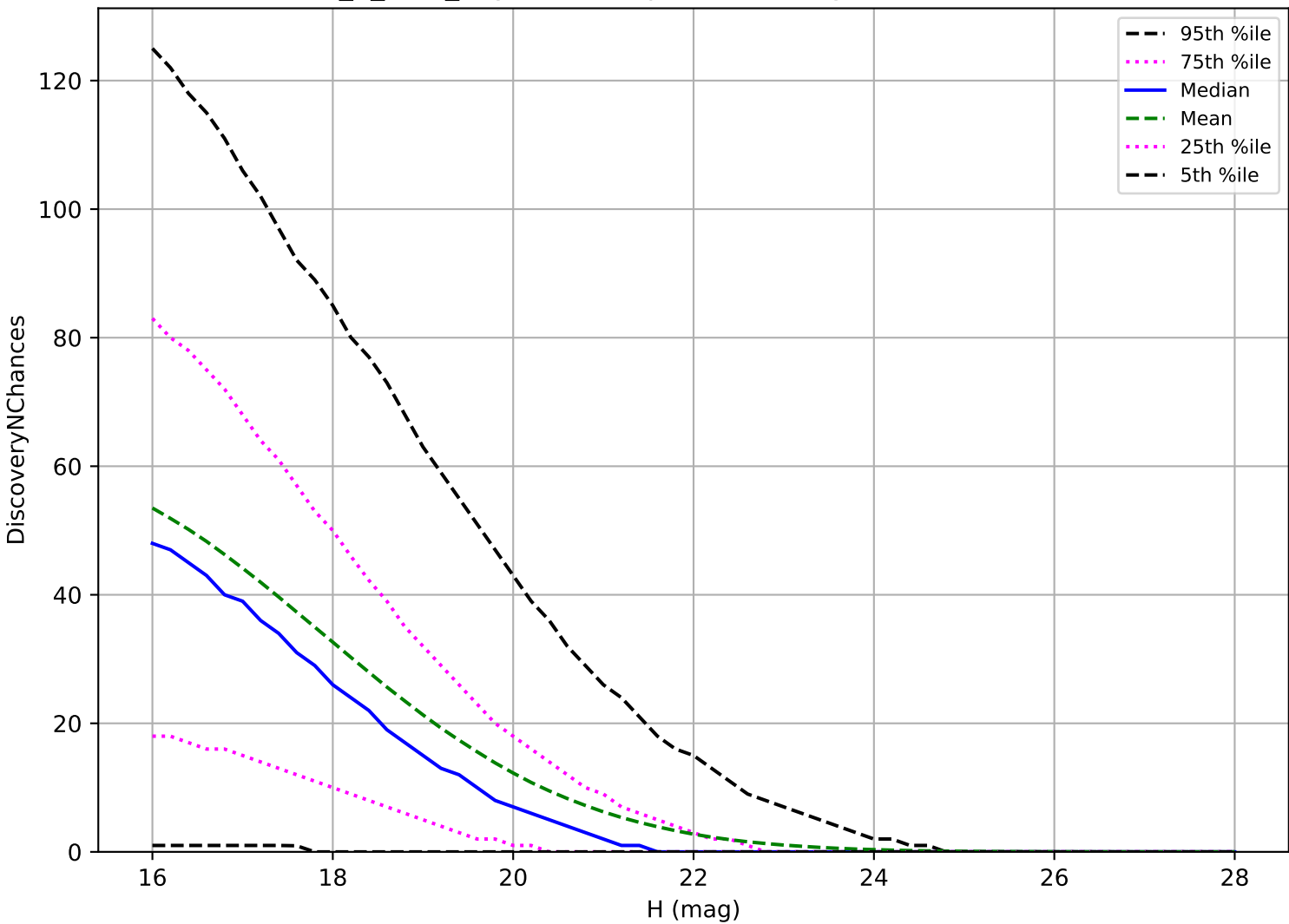
roll_3_v3.4_10yrs: PHA 3 pairs in 15 nights detection loss
