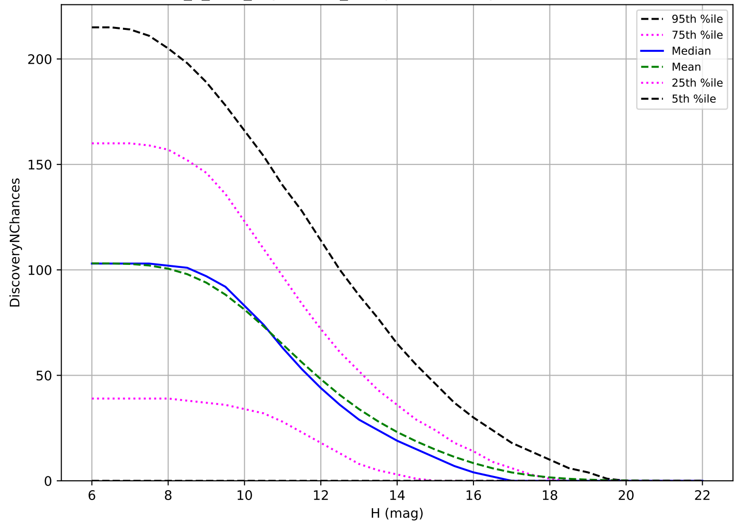
roll_3_v3.4_10yrs: OCC_r5 3 pairs in 15 nights detection loss
