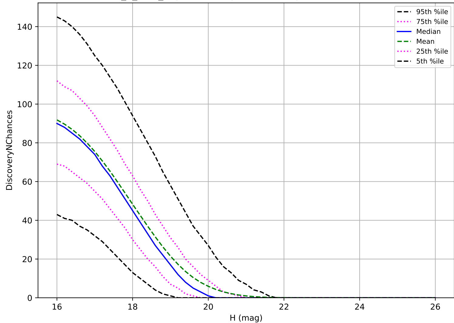
roll_3_v3.4_10yrs: MBA 3 pairs in 15 nights detection loss
