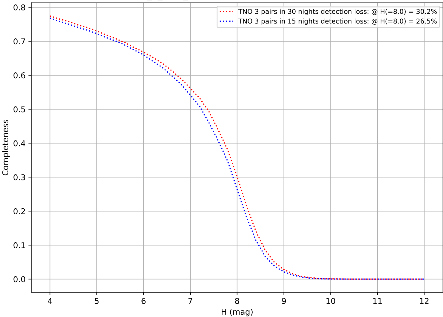
roll_3_v3.4_10yrs: DifferentialCompleteness
