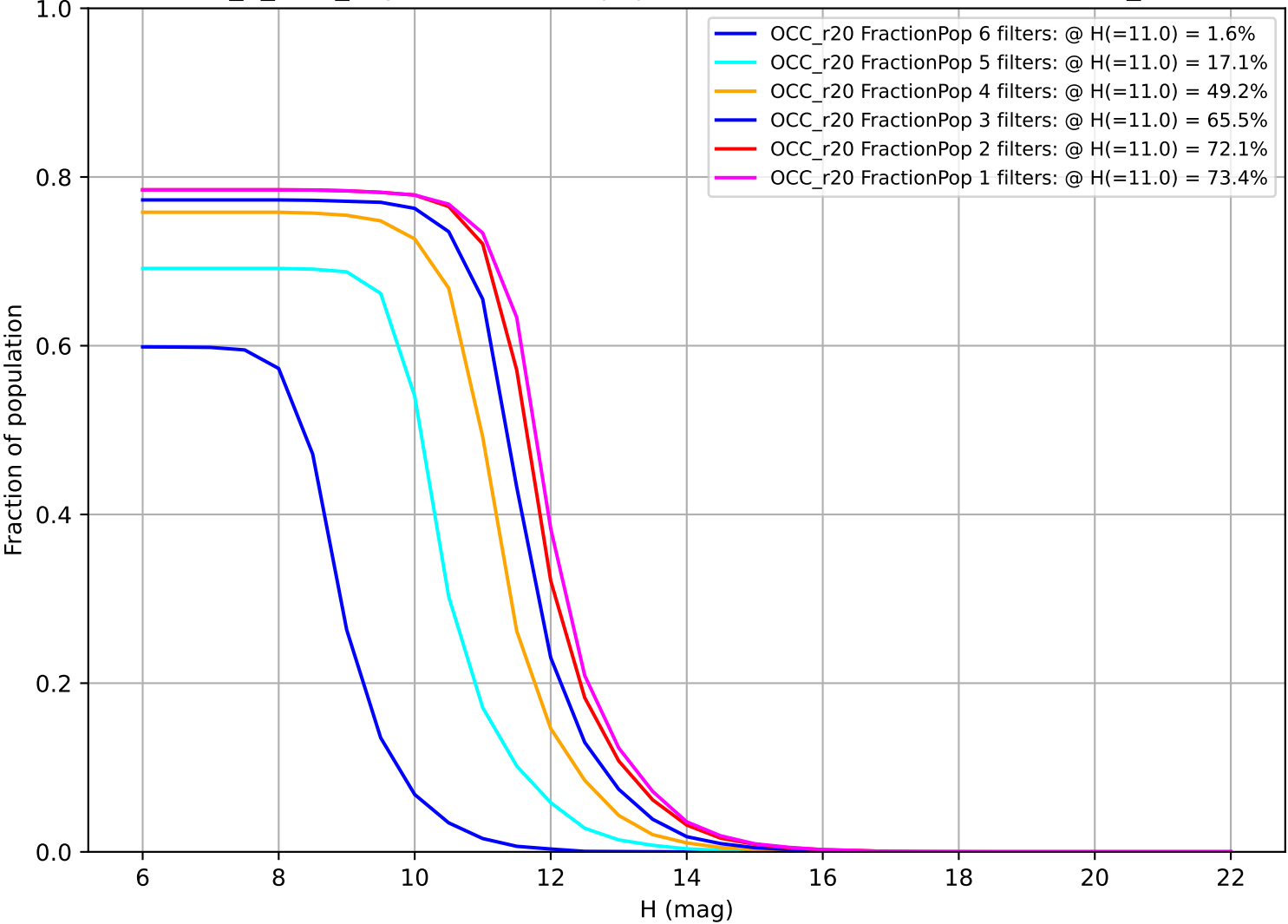
roll_3_v3.4_10yrs: Fraction of population with colors in X filters OCC_r20
