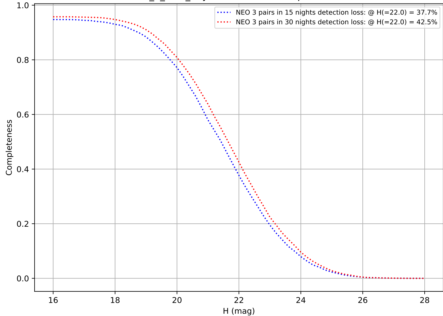
roll_3_v3.4_10yrs: DifferentialCompleteness
