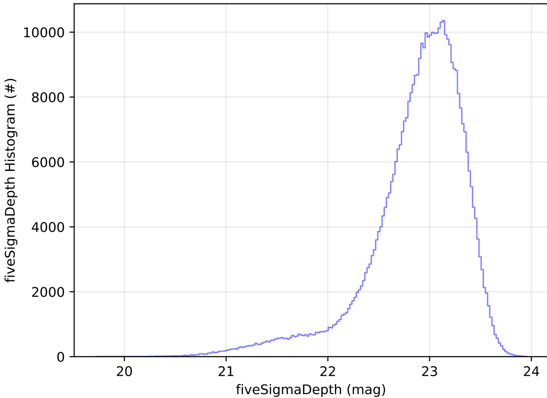
roll_3_v3.4_10yrs z: fiveSigmaDepth Histogram
