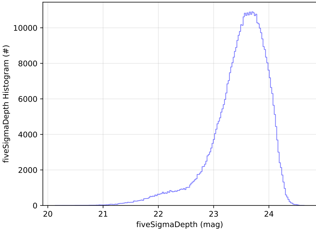
roll_3_v3.4_10yrs i: fiveSigmaDepth Histogram
