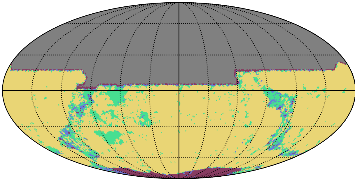
roll_3_v3.4_10yrs y band: YearCoverage night
