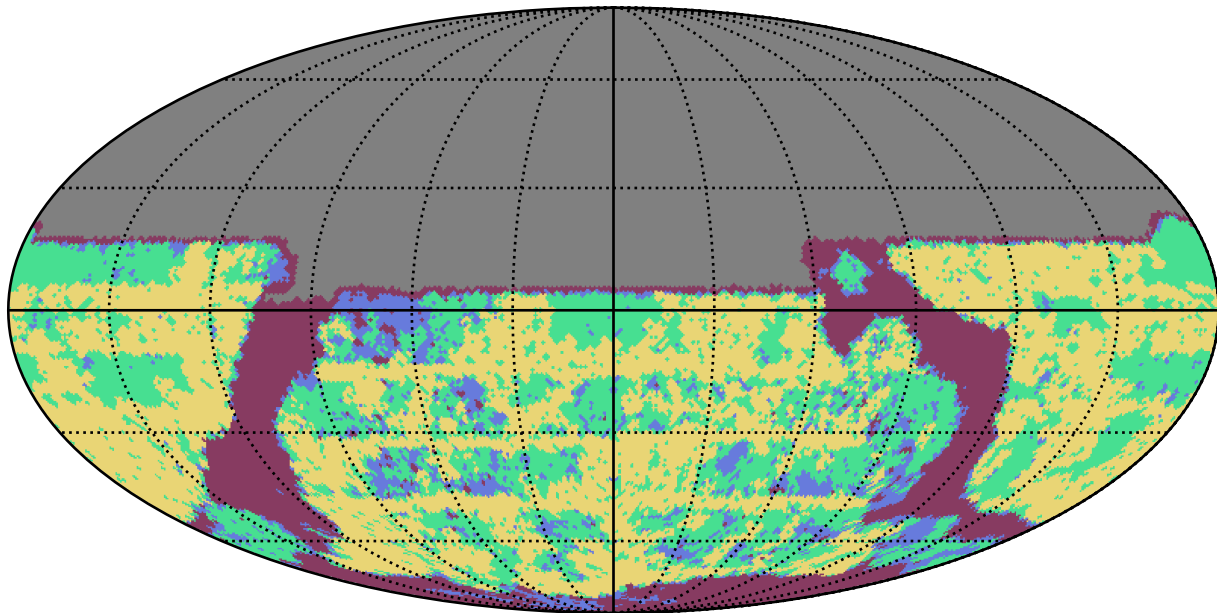
roll_3_v3.4_10yrs u band: YearCoverage night
