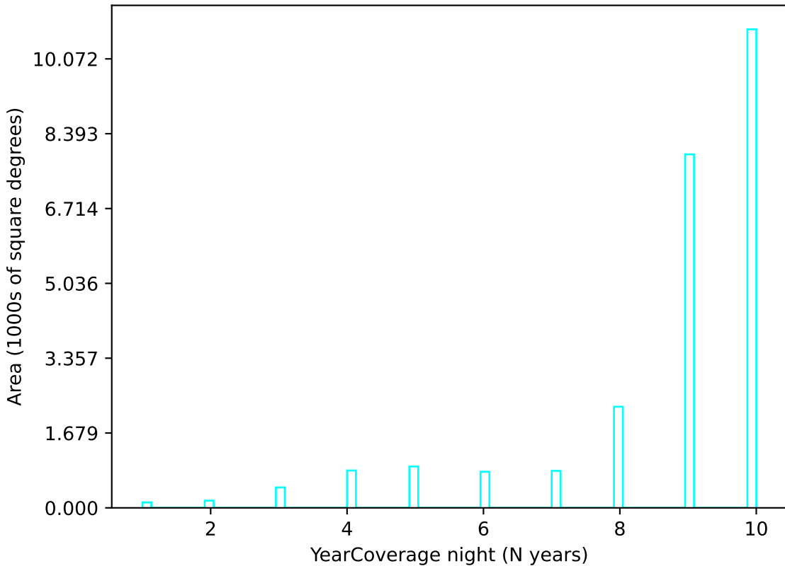
roll_3_v3.4_10yrs u band: YearCoverage night
