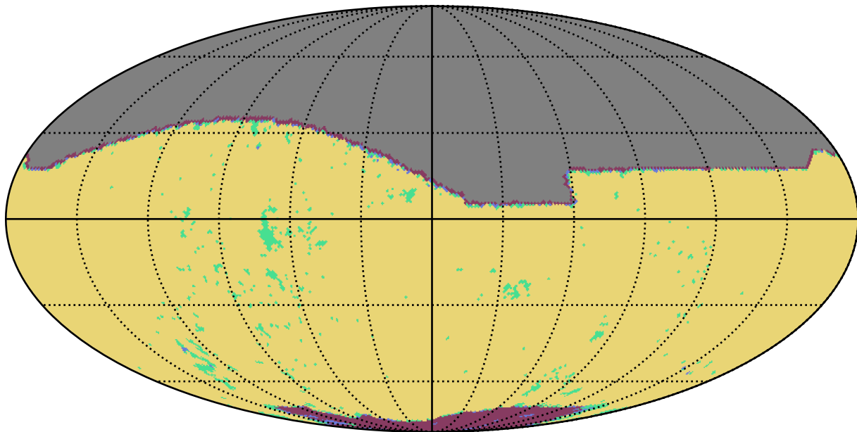
roll_3_v3.4_10yrs r band: YearCoverage night
