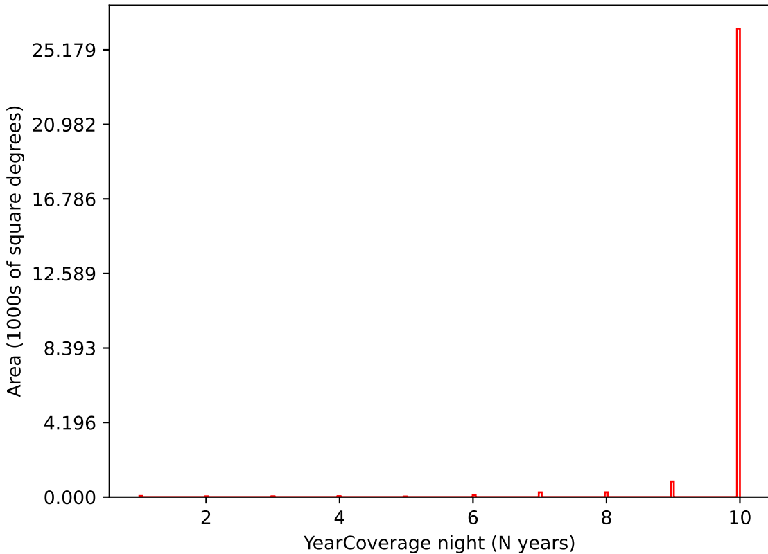
roll_3_v3.4_10yrs i band: YearCoverage night
