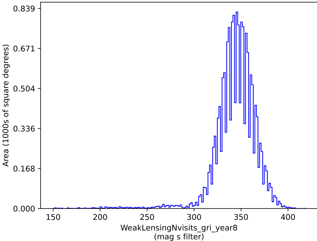
roll_3_v3.4_10yrs gri band non-DD: WeakLensingNvisits_gri_year8
