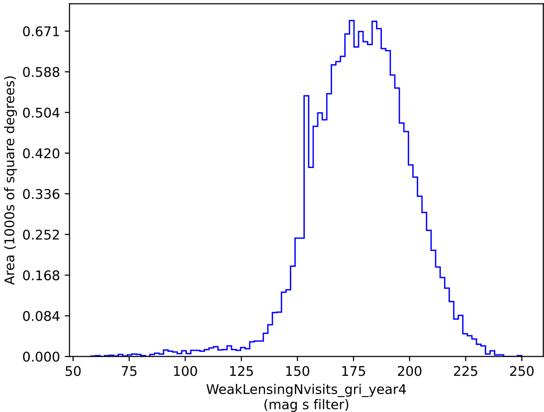
roll_3_v3.4_10yrs gri band non-DD: WeakLensingNvisits_gri_year4
