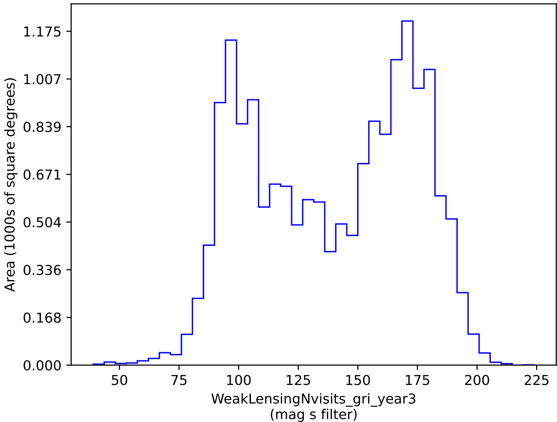
roll_3_v3.4_10yrs gri band non-DD: WeakLensingNvisits_gri_year3
