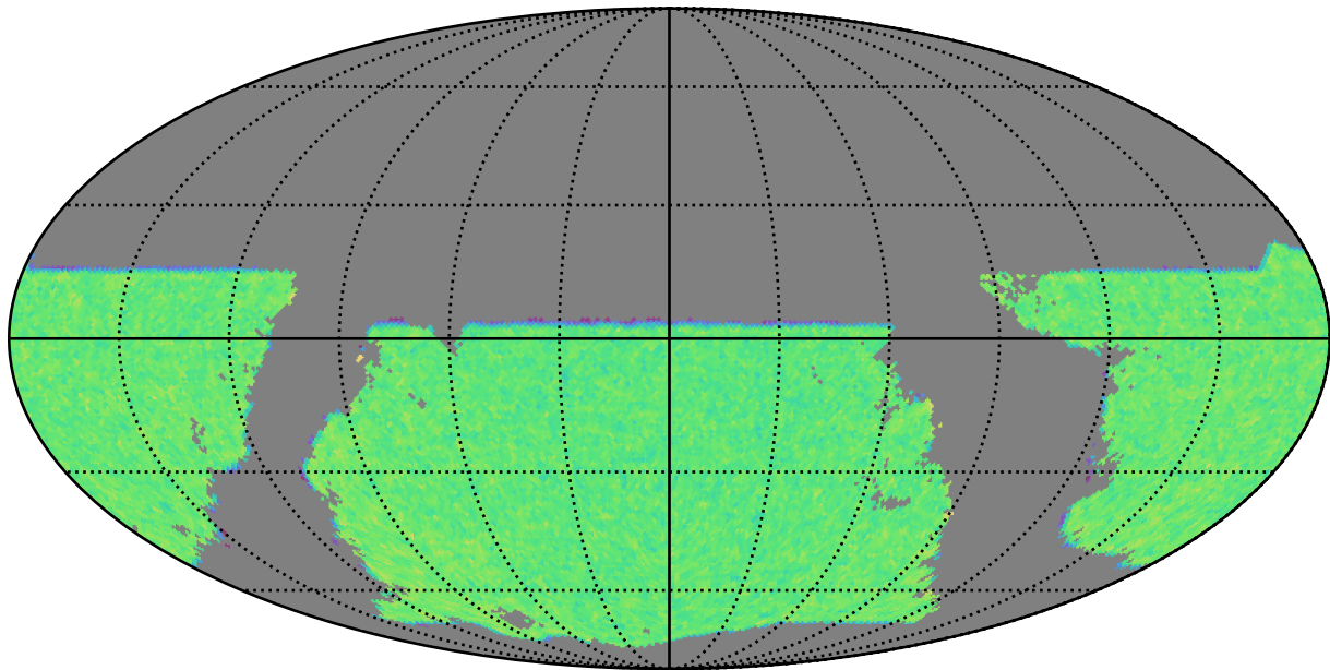
roll_3_v3.4_10yrs gri band non-DD: WeakLensingNvisits
