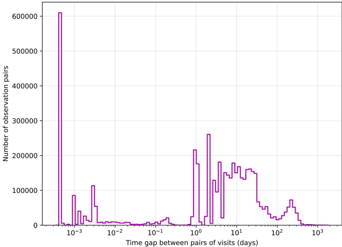
roll_3_v3.4_10yrs z band: Tgaps observationStartMJD
