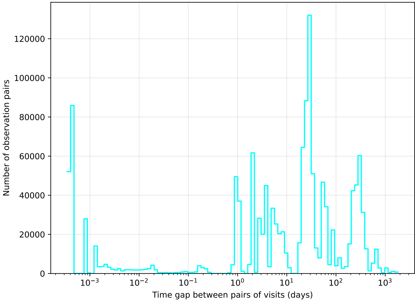
roll_3_v3.4_10yrs u band: Tgaps observationStartMJD
