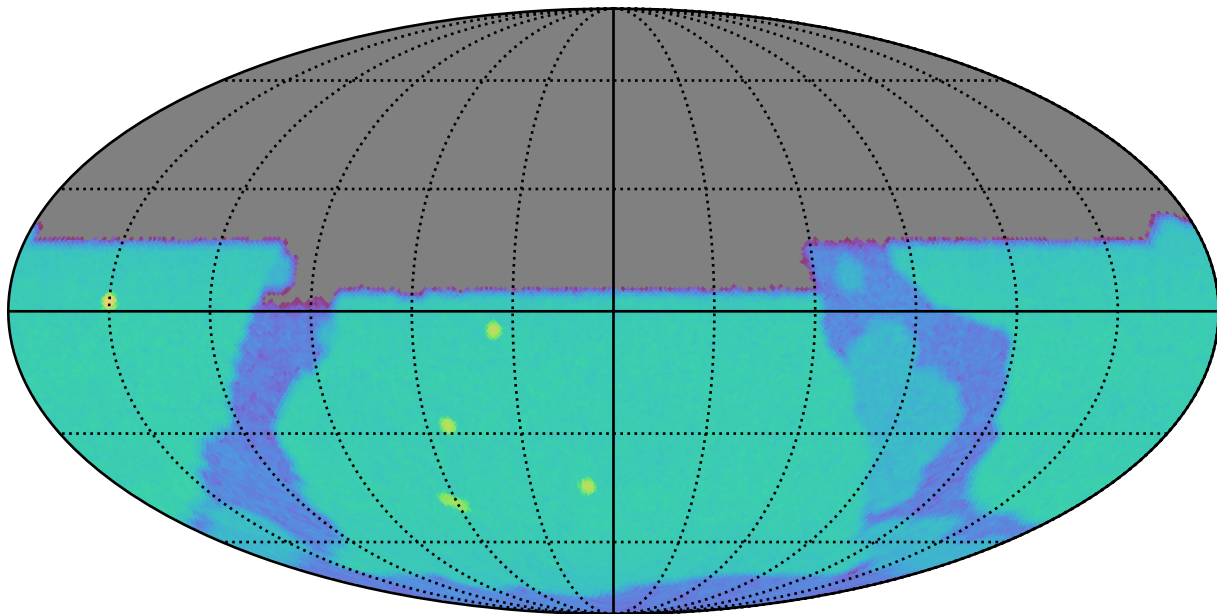
roll_3_v3.4_10yrs u: SurfaceBrightLimit
