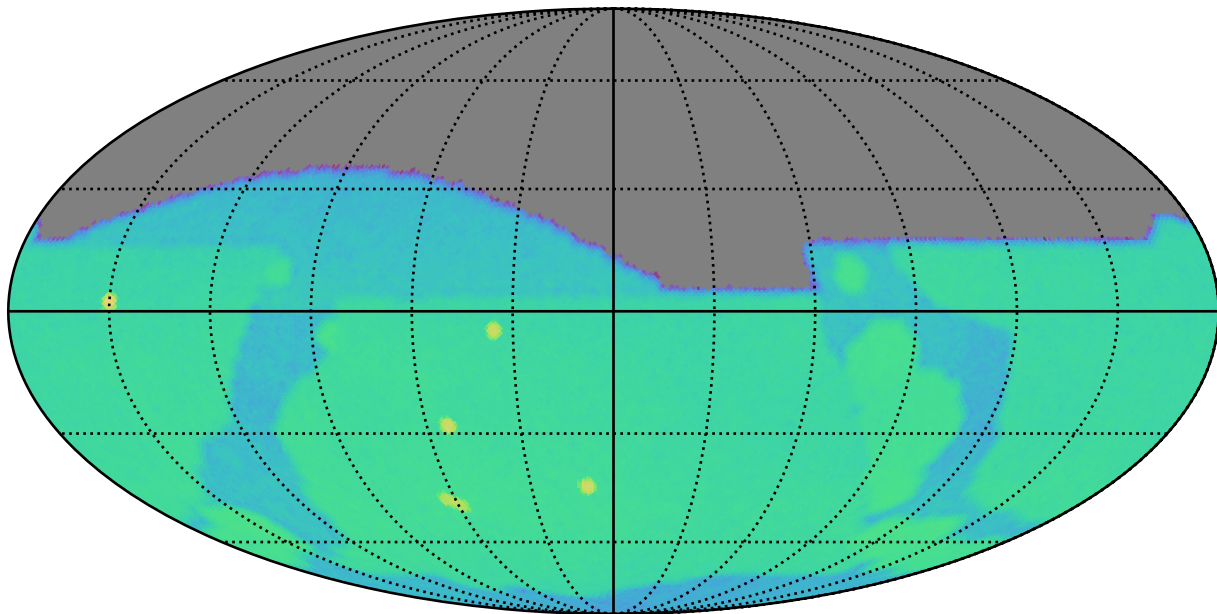
roll_3_v3.4_10yrs g: SurfaceBrightLimit
