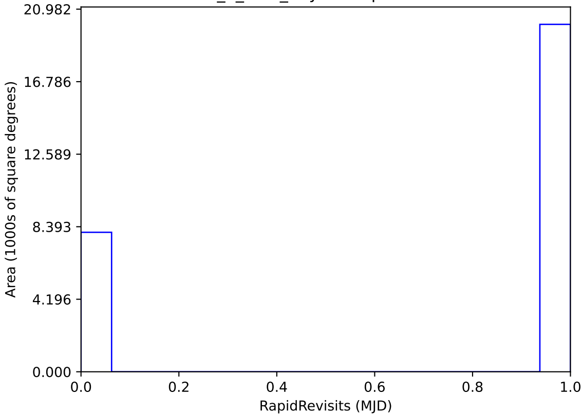
roll_3_v3.4_10yrs : RapidRevisits
