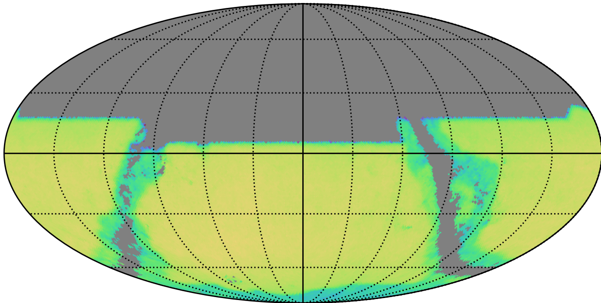
roll_3_v3.4_10yrs y band and non-DD: QSONumberCountsMetric
