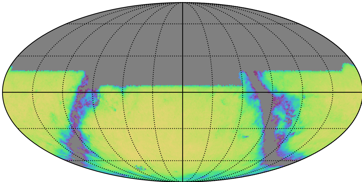
roll_3_v3.4_10yrs u band and non-DD: QSONumberCountsMetric
