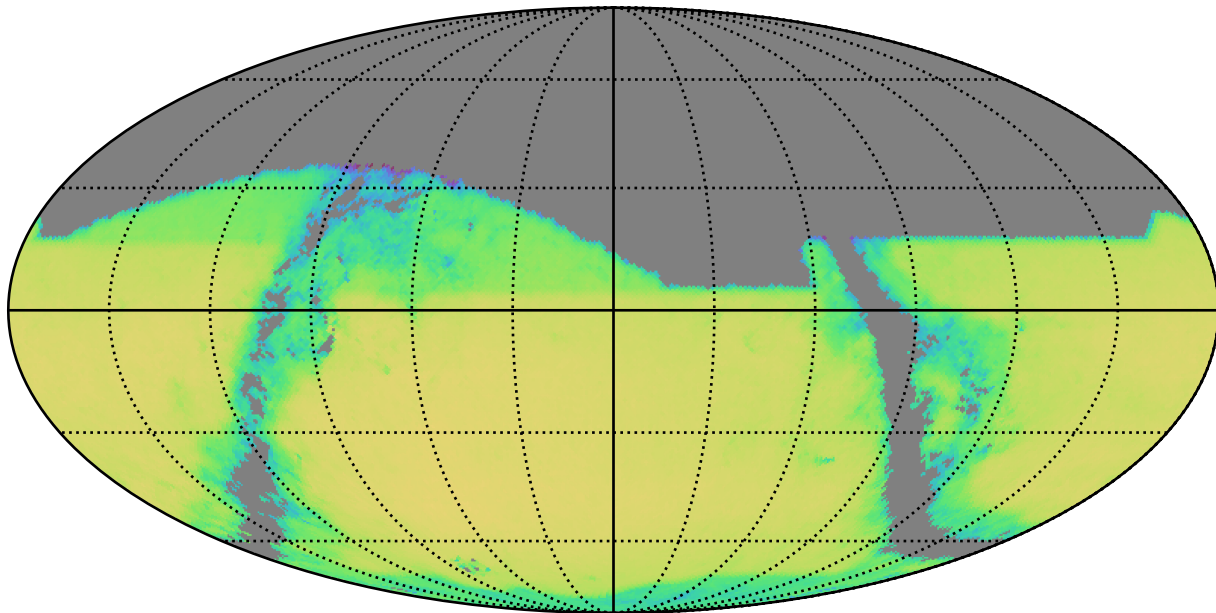
roll_3_v3.4_10yrs r band and non-DD: QSONumberCountsMetric
