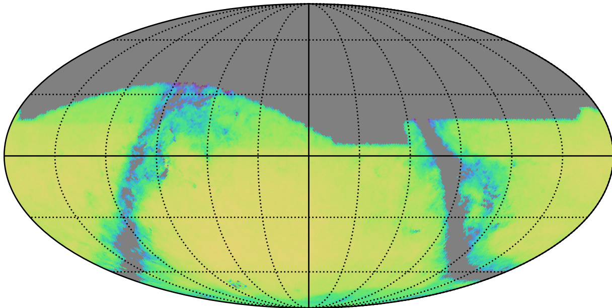
roll_3_v3.4_10yrs g band and non-DD: QSONumberCountsMetric
