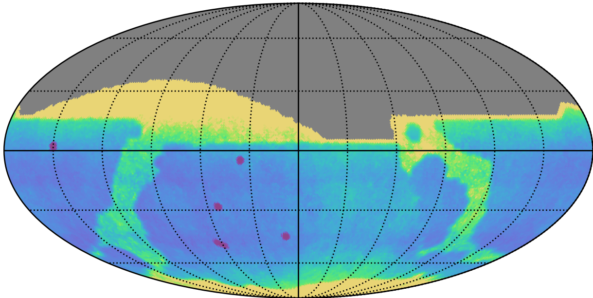
roll_3_v3.4_10yrs : Proper Motion Uncert @ 24.0
