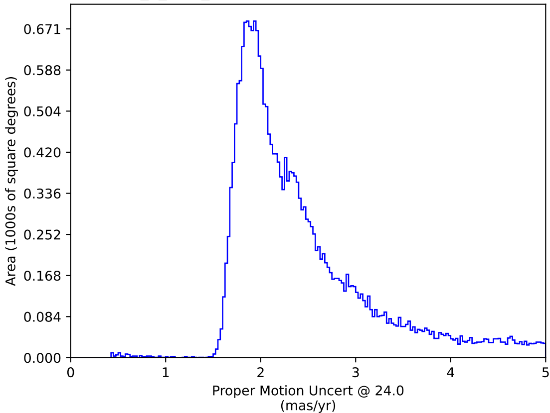
roll_3_v3.4_10yrs : Proper Motion Uncert @ 24.0
